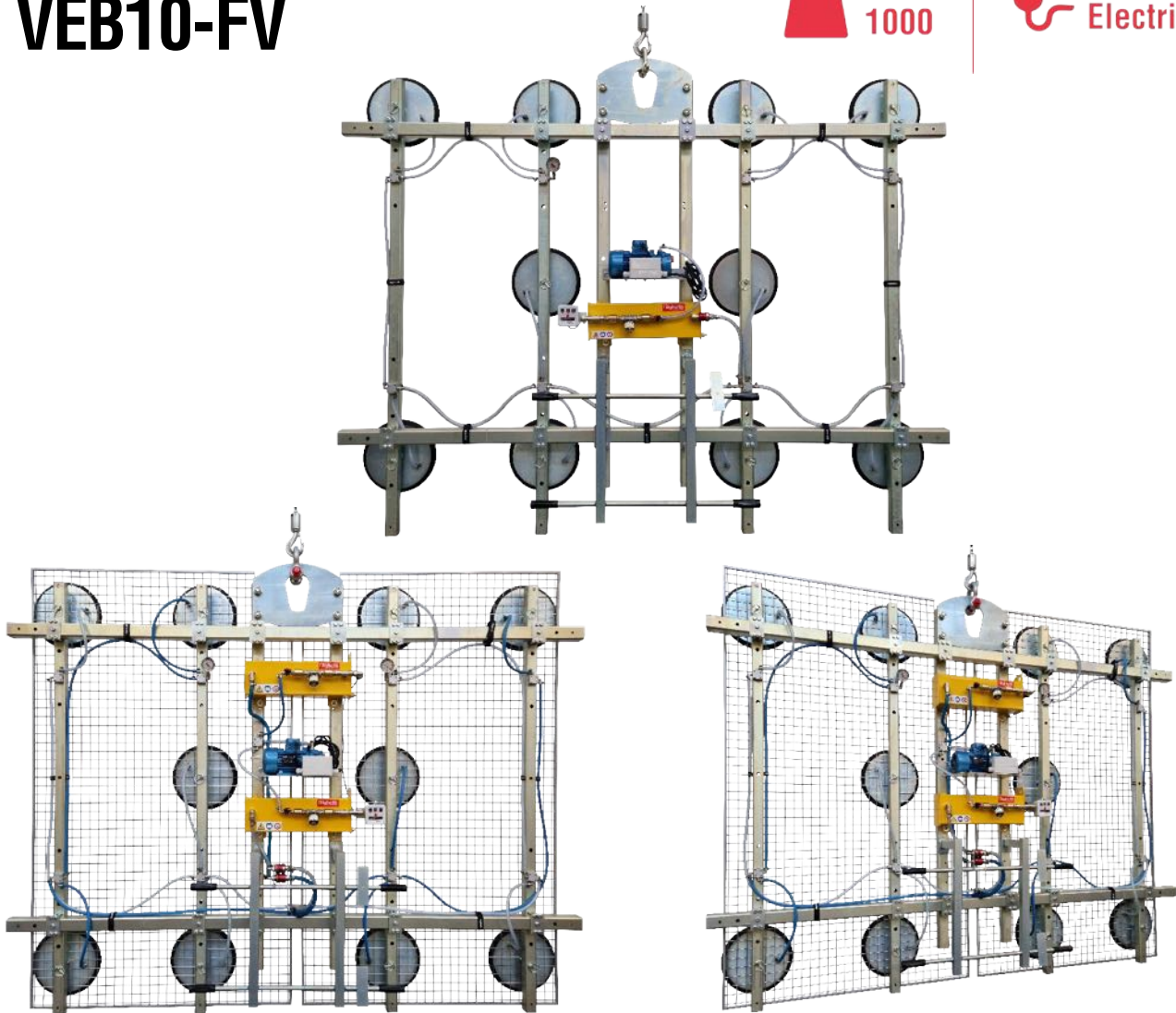
Picture: VEB10-FV with optional protection guard and dual vacuum circuit
